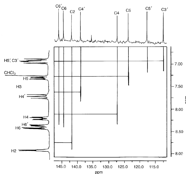
Fig. 7 HETCOR spectrum (contour plot) of 1 in \text{CDCl}_3
