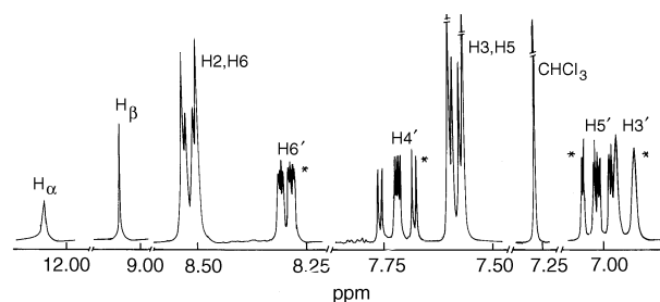
Fig. 4 Resolution enhanced ^1\text{H} NMR spectrum of 3 in CDCl 3
