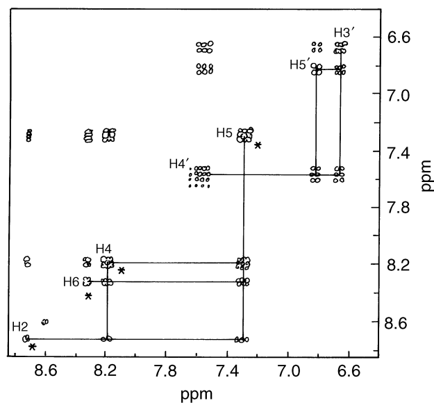
Fig. 3 COSY spectrum (contour plot) of 2 in CDCl 3 on 200 MHz spectrometer
