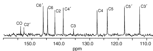
Fig. 6 ^{13}\text{C}\{-^1\text{H}\} NMR spectrum of 1 in \text{CDCl}_3
